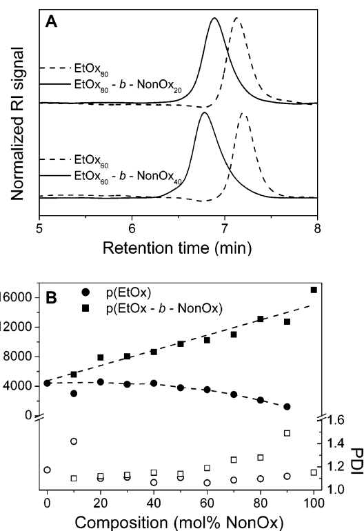
Figure 4. (A) Selected SEC traces of the EtOx polymers (first block) and the corresponding EtOx- b -NonOx copolymers with different amounts of NonOx content (SEC eluent: \text{CHCl}_3 with 2% isopropanol and 4% triethylamine). (B) M_n and PDI values of the EtOx- b -NonOx copolymers resulting from SEC analysis.
