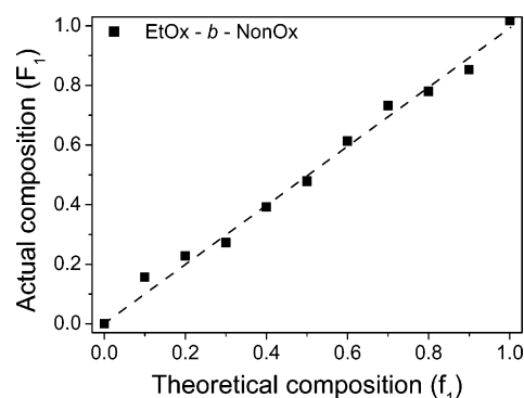
Figure 5. Actual composition plotted against theoretical composition, measured by ^1\text{H} NMR for the EtOx- b -NonOx copolymers.
