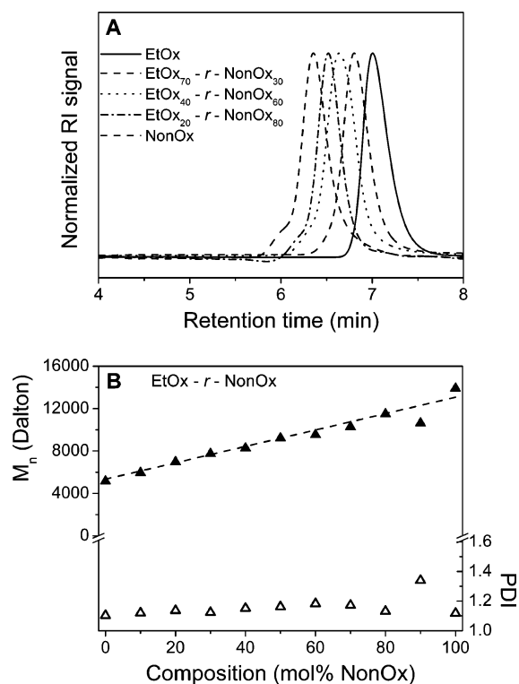
Figure 2. (A) Selected SEC traces of EtOx- r -NonOx copolymers with different amounts of NonOx content (SEC eluent: \text{CHCl}_3 with 2% isopropanol and 4% triethylamine). (B) M_n and PDI values of the EtOx- r -NonOx copolymers resulting from SEC analysis.
